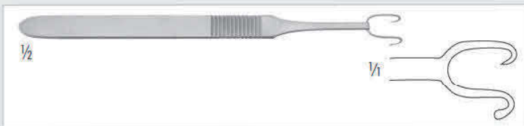
230-282-140 COTTLE Nasenflügelretractor, 2 Zinken, spitz/stumpf, 140 mm Alar retractor, 2 prongs, sharp/blunt, 5 1/2 inch
